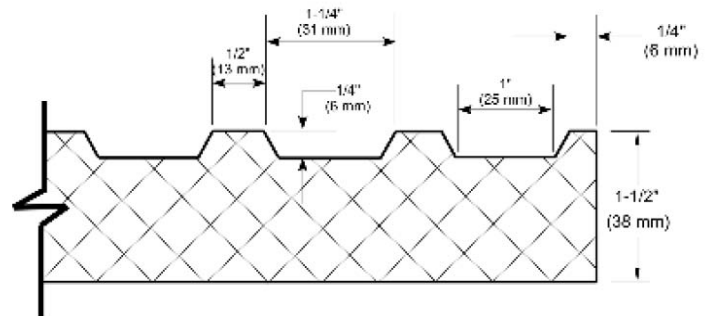
FIGURE 2—INSULATION BOARD
