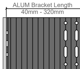
StoVentro ALUM - Small Bracket (GP) with Thermal Blocking Element
