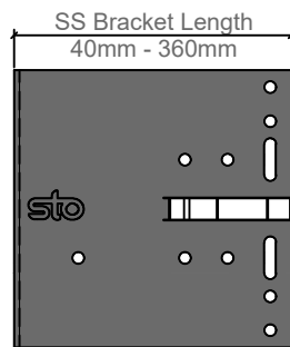
StoVentro SS - Large Bracket (FP)
