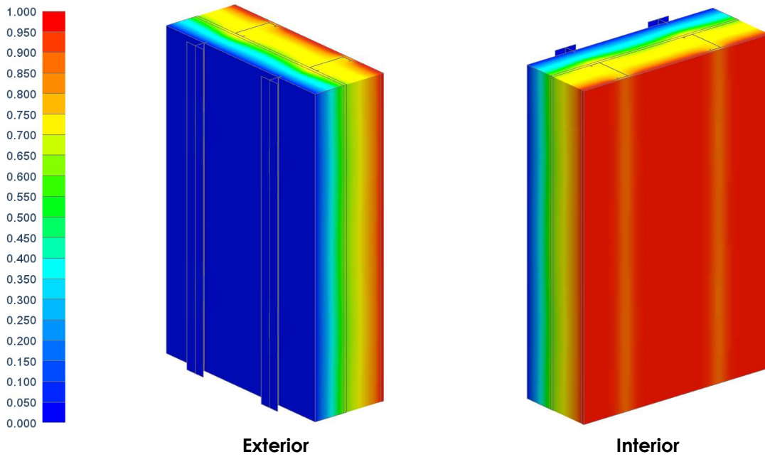
Figure E5: Temperature Profile Stainless Steel 160 GP Bracket with Split Insulated Steel Stud
