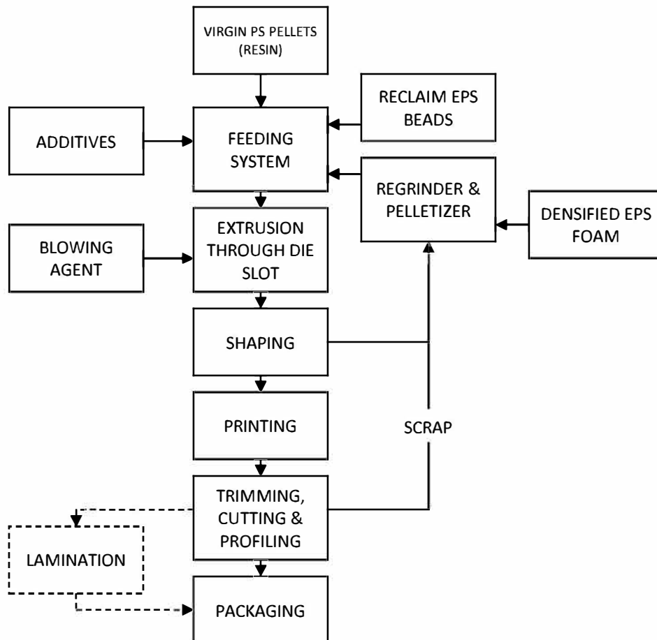
Figure 1. Process Flow Diagram for Manufacturing of XPS Insulation
