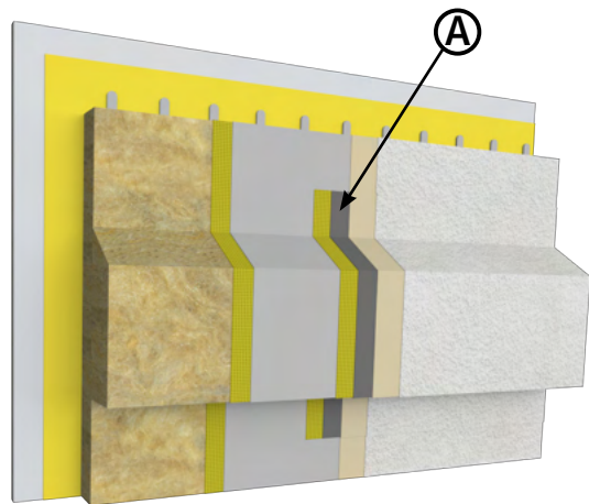
Thick Build Out with Added Waterproofing Component (A)
